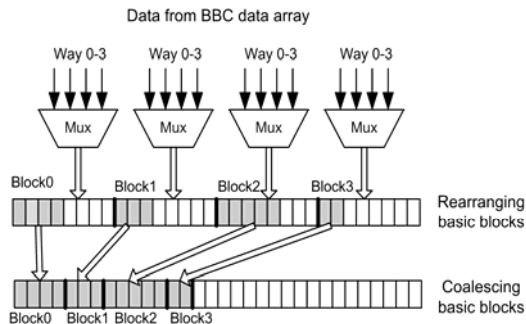
Figure 4: Coalescing Buffer
